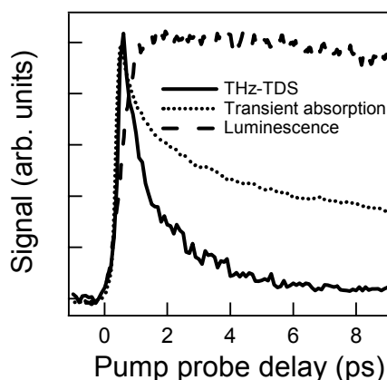
Figure 7.4 Dynamics of THz field modulation (full line, measured at the peak of the THz pulse at t=1.2 ps), transient absorption intensity (dotted line, measured with 800 nm probe pulse) and luminescence intensity (up-converted with 800 nm pulse), after excitation with a 400 nm excitation pulse. Signals have been normalized to peak height.
