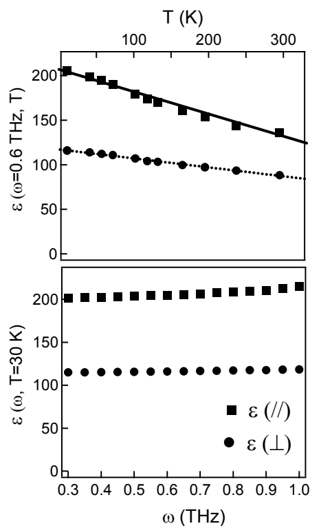
Figure 4.3 Upper panel: Temperature dependence of the real part of lattice dielectric function ( \epsilon ) at 0.6 THz, extracted from E_{free}(t) and E_{trans}(t) , with the THz polarization parallel ( // ) or perpendicular ( \perp ) to the c axis of the crystal. Only the real parts are plotted, since the imaginary parts negligibly small (more than two orders of magnitude smaller). The largest dielectric function is measured in the direction parallel to the c axis, though the anisotropy decreases slightly with temperature. Lower panel: Frequency dependence of the dielectric function at 30K, which is almost completely flat over this frequency range in the perpendicular direction, and increasing slightly with frequency in the parallel direction. The shape of the frequency dependence is similar at all temperatures. The lines drawn through the data in the upper panel (straight line fits yielding \epsilon_{//}=207-0.265\times T and \epsilon_{\perp}=117-0.101\times T ) are to guide the eye.
