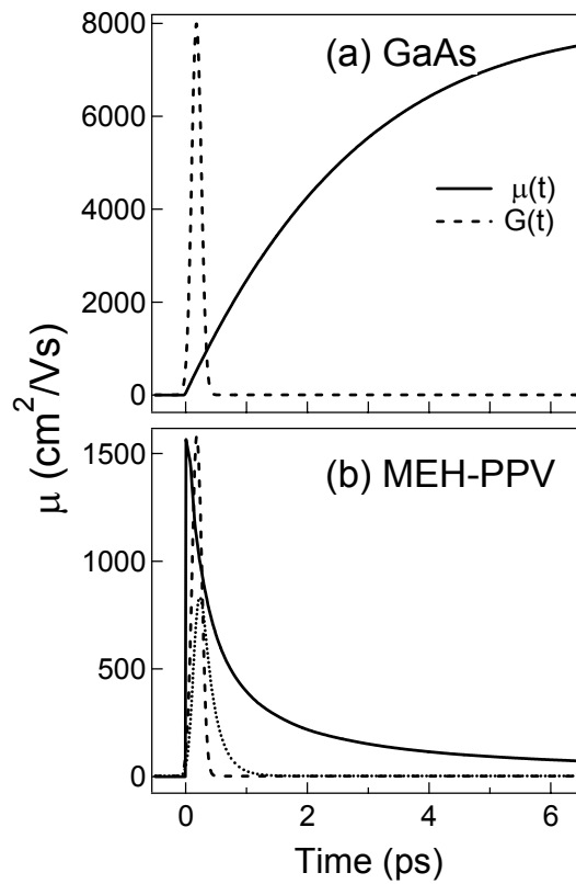
Figure 7.12 Comparison of timescales involved in charge generation and cooling; the solid lines in both figures represent the calculated time dependent mobility, \mu(t) , in (a) GaAs (excitation with 400 nm, calculated using the formalism introduced in Ref. [74]) and (b) MEH-PPV (calculated from Ref. [53] – see text). Dashed lines represent the generation rate, G(t) , assuming instantaneous generation of charges upon excitation, i.e. described by the Gaussian intensity profile of the excitation pulse (FWHM 180 fs). The dotted line in (b) describes the generation rate for charges generated from hot excitons with a dissociation rate of (200 \text{ fs})^{-1} (see text). In (a) the rise in photocurrent is dominated by the slow evolution in \mu(t) , while in (b) the rise in G(t) and decay in \mu(t) occur on the same timescale.
