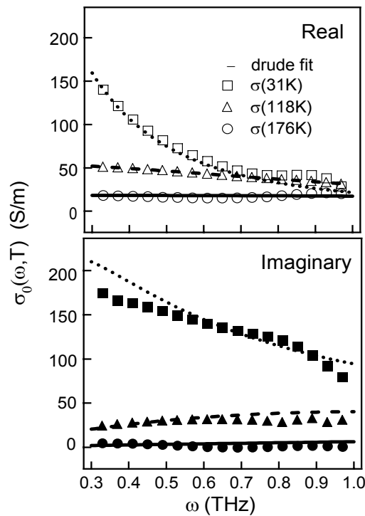
Figure 4.4 Pump (400 nm) induced complex conductivity at the sample interface (real parts plotted as hollow symbols, imaginary parts as filled symbols) measured perpendicular to the c axis for three different temperatures. The Drude model describes the data very well (lines), with one scattering time for both real and imaginary response at each temperature. A similar response is observed perpendicular to the c axis.
